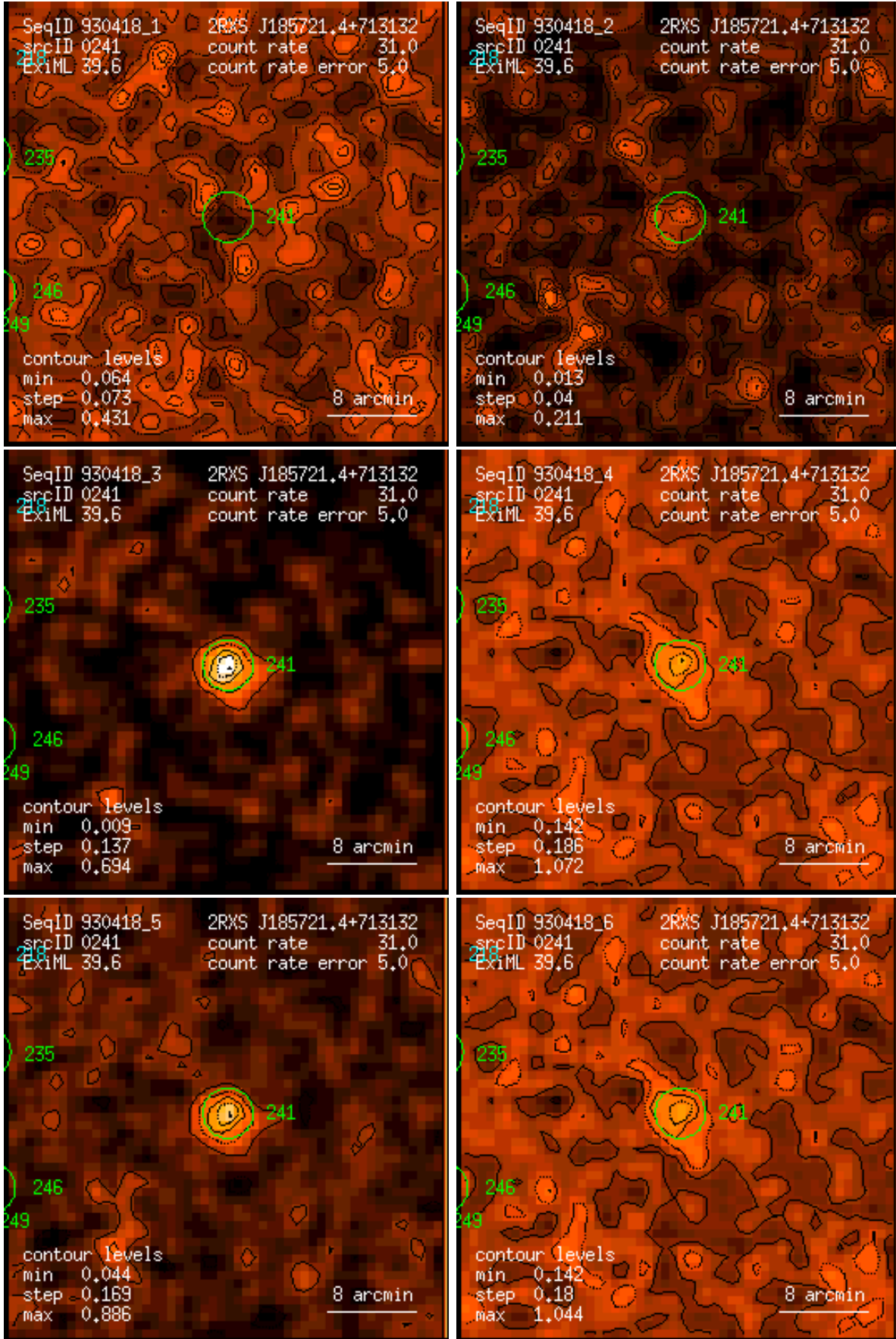
Figure 241: RASS 930418: detection 0241: band rate images, Gaussian filter: (1) PSPC channels 11 – 41, (2) 52 – 90, (3) 91 – 201, (4) 11 – 235, (5) 52 – 201, (6) 11 – 201. Broad band rates in counts/ks. Band rate contour levels in counts/ks/arcmin 2 .
