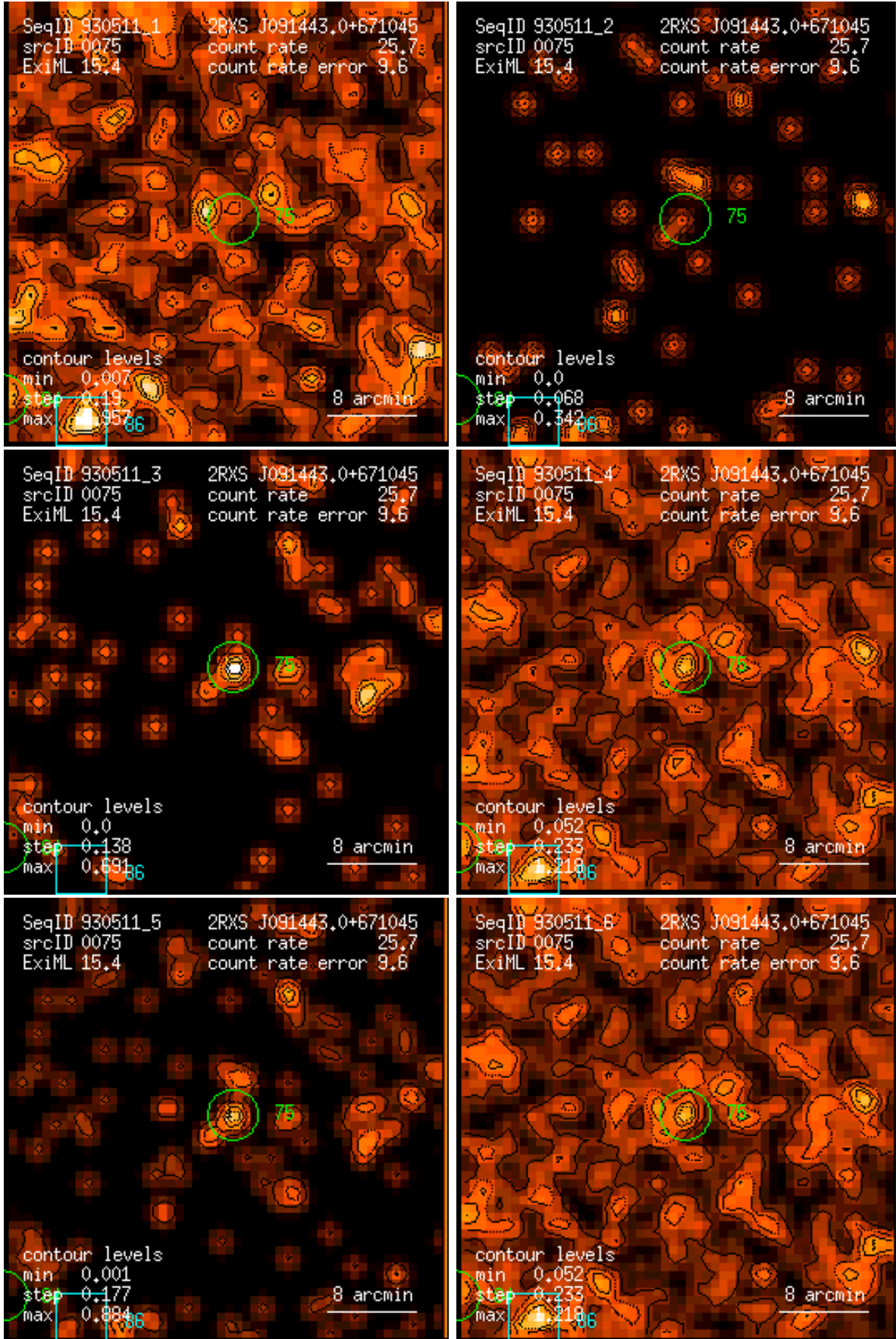
Figure 75: RASS 930511: detection 0075: band rate images, Gaussian filter: (1) PSPC channels 11 – 41, (2) 52 – 90, (3) 91 – 201, (4) 11 – 235, (5) 52 – 201, (6) 11 – 201. Broad band rates in counts/ks. Band rate contour levels in counts/ks/arcmin 2 .
