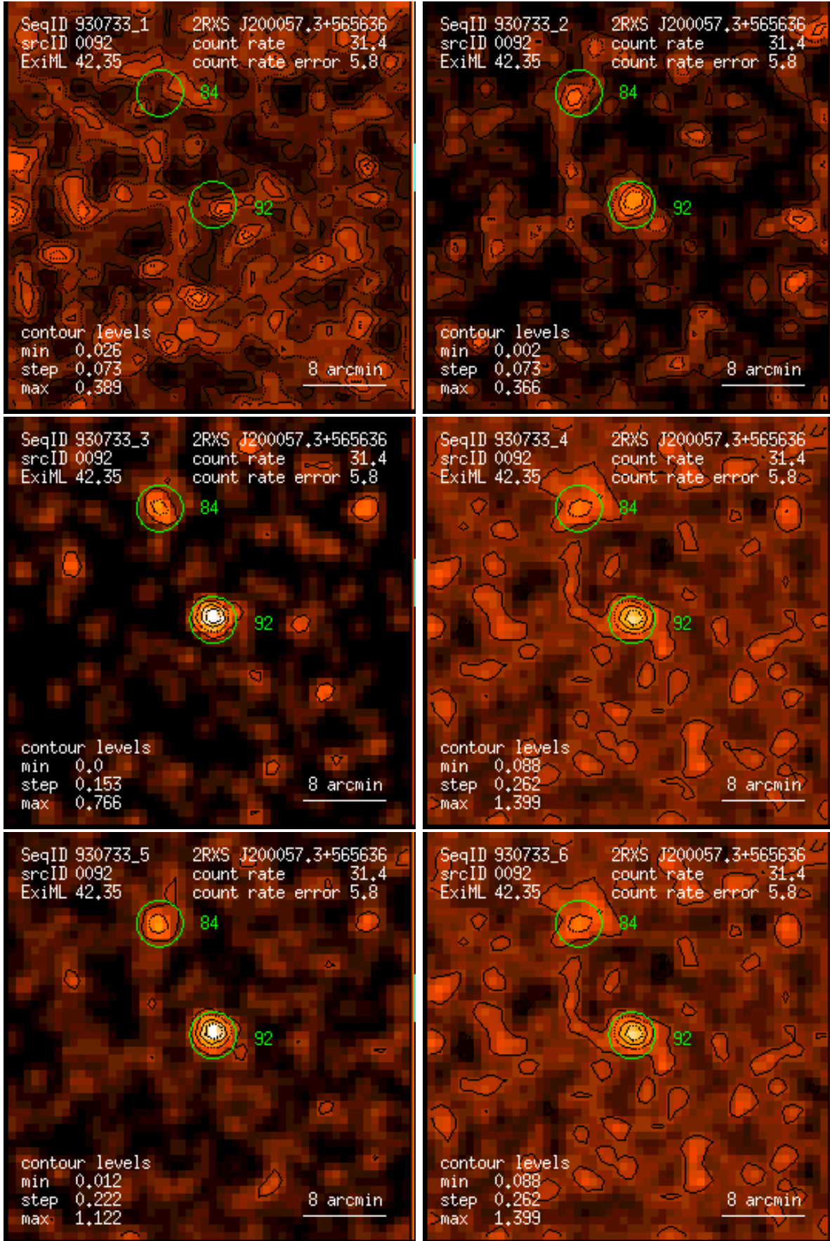
Figure 92: RASS 930733: detection 0092: band rate images, Gaussian filter: (1) PSPC channels 11 – 41, (2) 52 – 90, (3) 91 – 201, (4) 11 – 235, (5) 52 – 201, (6) 11 – 201. Broad band rates in counts/ks. Band rate contour levels in counts/ks/arcmin 2 .
