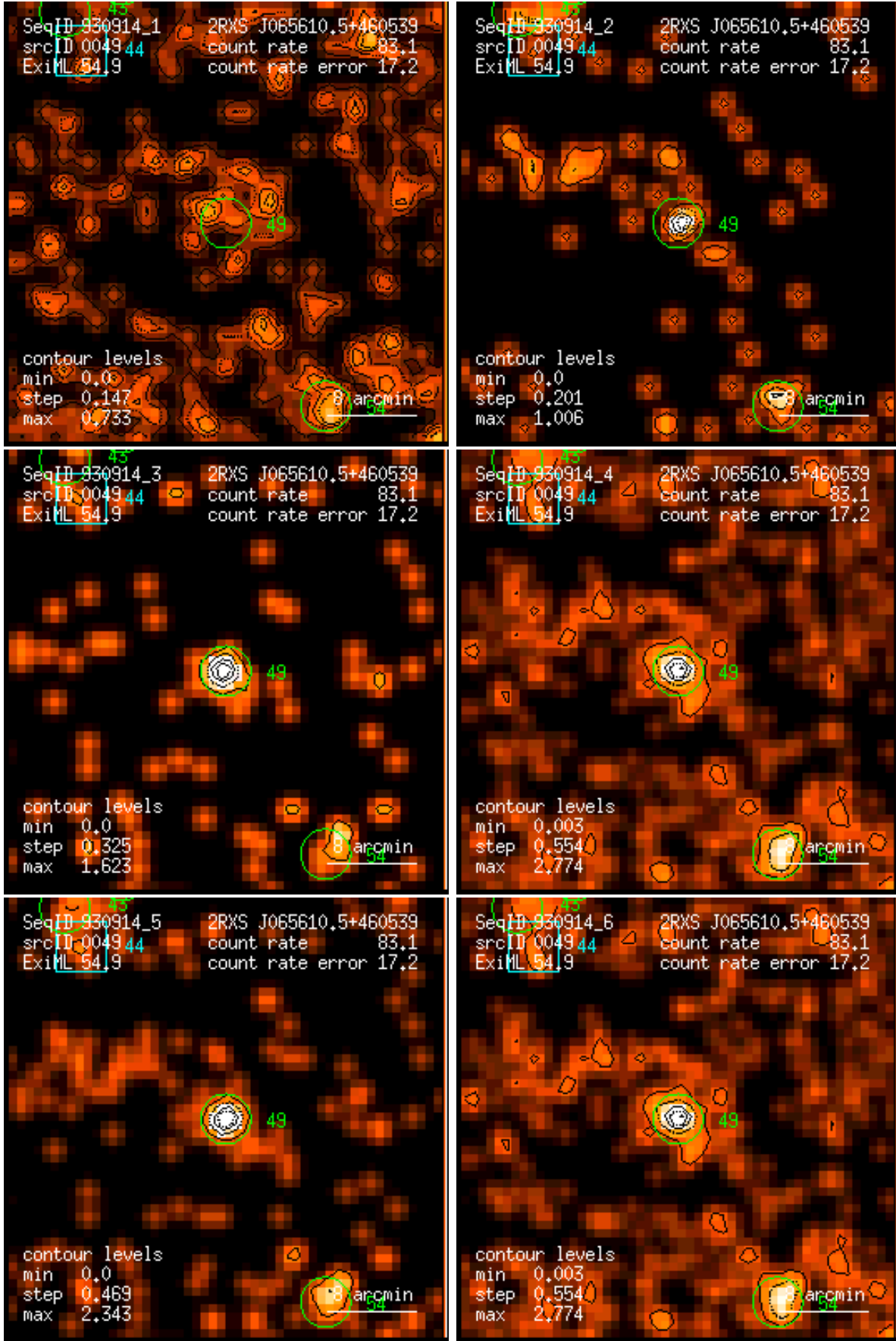
Figure 49: RASS 930914: detection 0049: band rate images, Gaussian filter: (1) PSPC channels 11 – 41, (2) 52 – 90, (3) 91 – 201, (4) 11 – 235, (5) 52 – 201, (6) 11 – 201. Broad band rates in counts/ks. Band rate contour levels in counts/ks/arcmin 2 .
