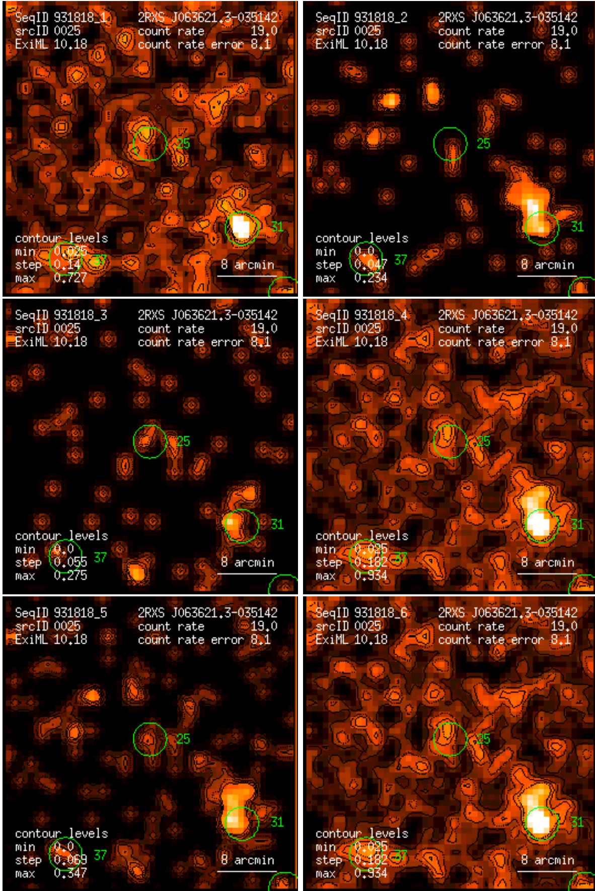
Figure 25: RASS 931818: detection 0025: band rate images, Gaussian filter: (1) PSPC channels 11 – 41, (2) 52 – 90, (3) 91 – 201, (4) 11 – 235, (5) 52 – 201, (6) 11 – 201. Broad band rates in counts/ks. Band rate contour levels in counts/ks/arcmin 2 .
