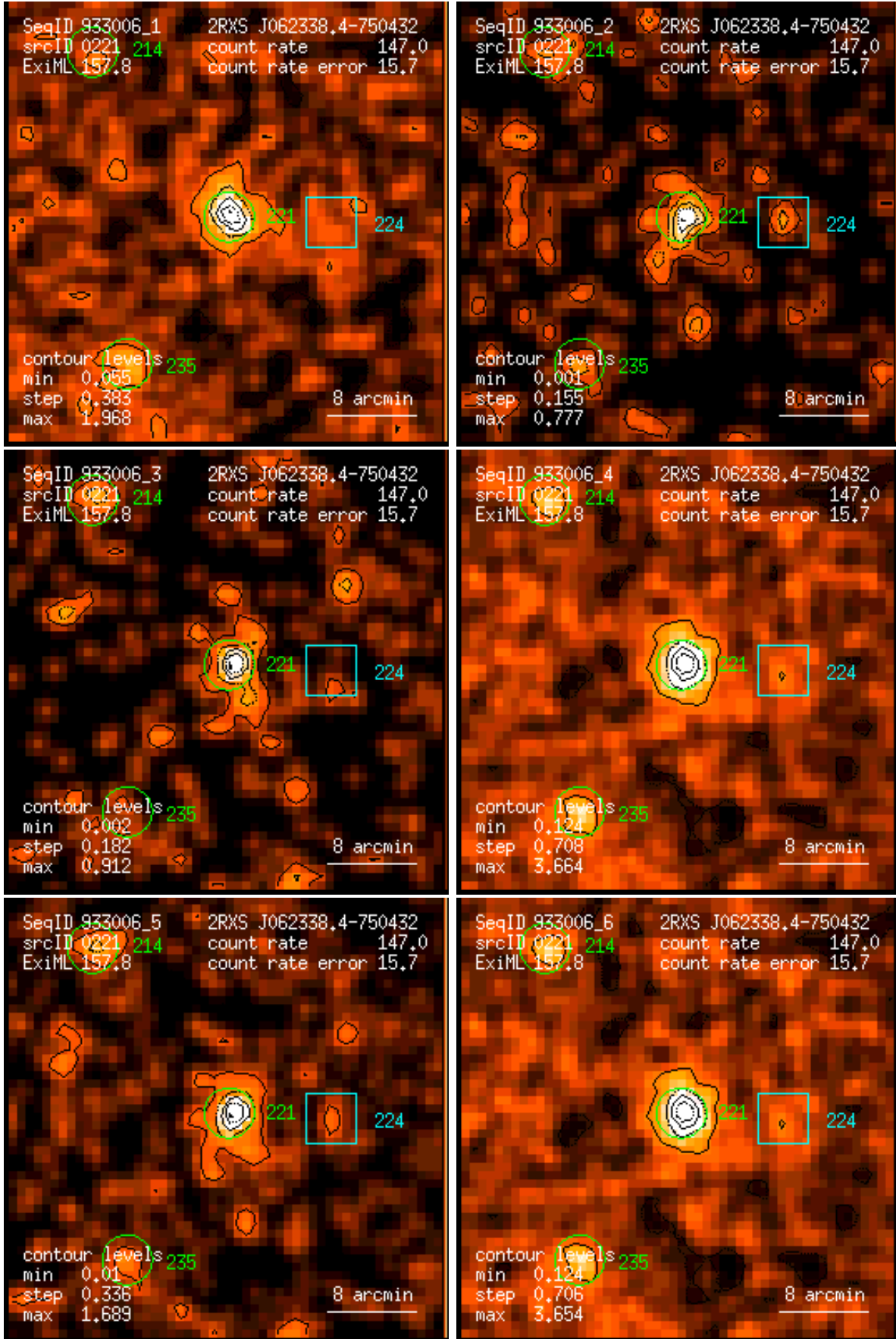
Figure 221: RASS 933006: detection 0221: band rate images, Gaussian filter: (1) PSPC channels 11 – 41, (2) 52 – 90, (3) 91 – 201, (4) 11 – 235, (5) 52 – 201, (6) 11 – 201. Broad band rates in counts/ks. Band rate contour levels in counts/ks/arcmin 2 .
